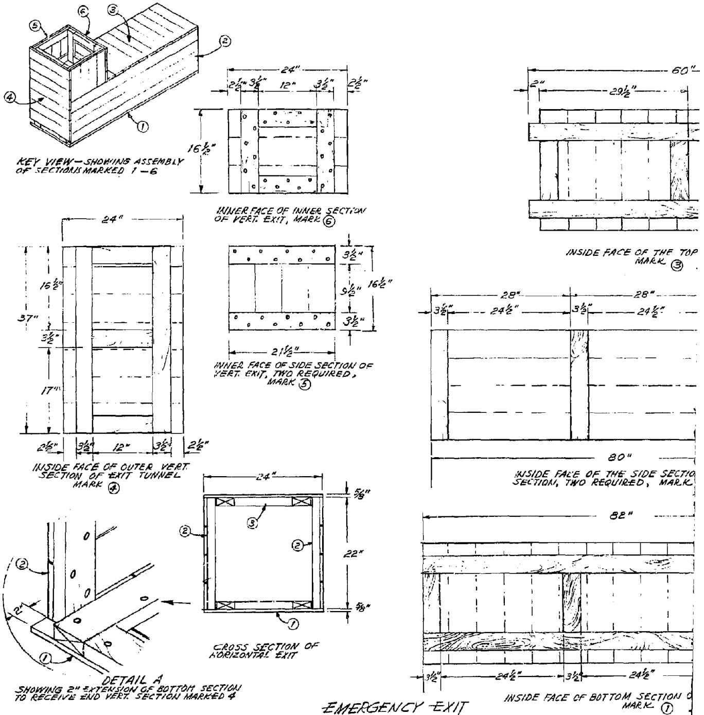
Fig. A-5.2. Shored Trench Stoop-In Shelter, Escape Hatch Details.
